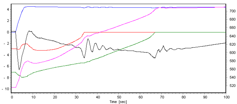
Legend for the graphs: - Discharge pump [m 3 /s] (Red line) - Discharge siphon pump [m 3 /s] (Green line) - Total discharge [m 3 /s] (Magenta line) - Discharge Pelton unit 2 [m 3 /s] (Blue line) - Head in penstock (2nd) [mWC] (Black line)
