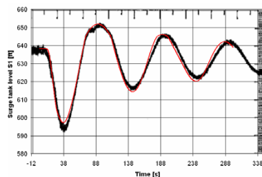
Turbine mode
