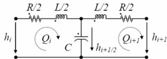
Figure 3 Equivalent circuit of an elementary pipe of length dx.
